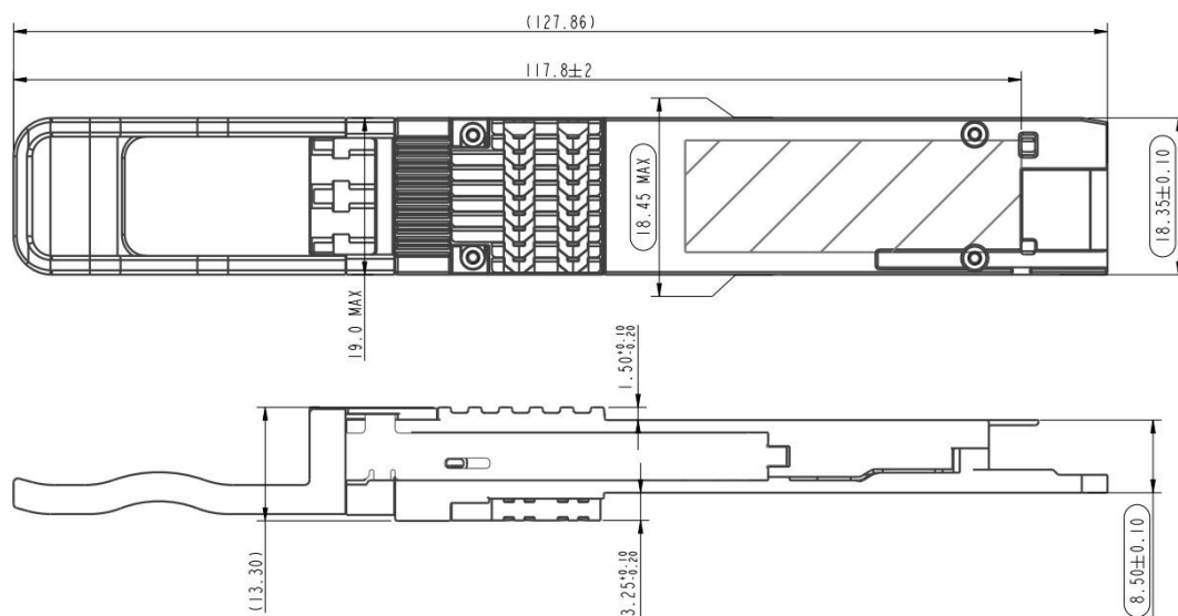
Figure 3. OM9660LS100 Mechanical Dimensions
